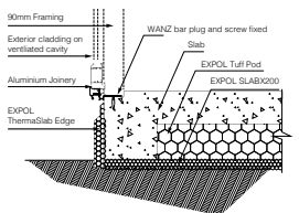
Waffle Pod Floor with WANZ Bar 90mm Framing/Cladding
