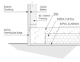
Waffle Pod Floor 90 - 140mm Framing/Lightweight Cladding/MaxEdge
