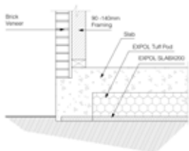
Waffle Pod Floor 90 - 140mm Framing/Brick Veneer/MaxEdge
