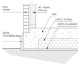
Waffle Pod Floor 90 - 140mm Framing/Brick Veneer
