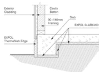
Slab on Grade with Footing 90 -140mm Framing/Cladding
