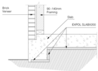
Slab on Grade with Footing 90 -140mm Framing/Brick Veneer
