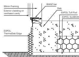
Waffle Pod Floor with WANZ Bar 90mm Framing/Cladding
