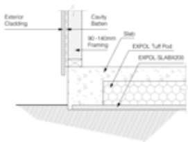
Waffle Pod Floor 90 - 140mm Framing/Cladding
