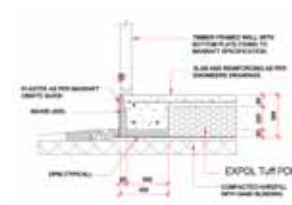
Waffle Pod Floor 90 - 140mm Framing/Lightweight Cladding/MaxEdge
